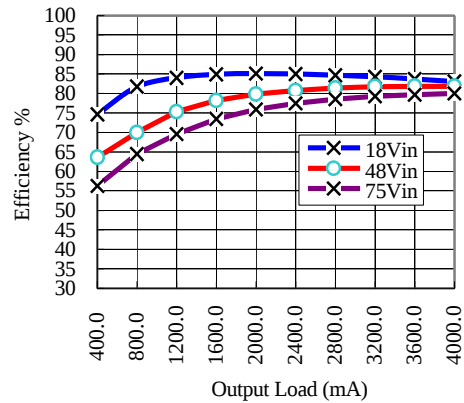
Efficiency vs. Load @ +25° Ambient, AEE04F36-L
